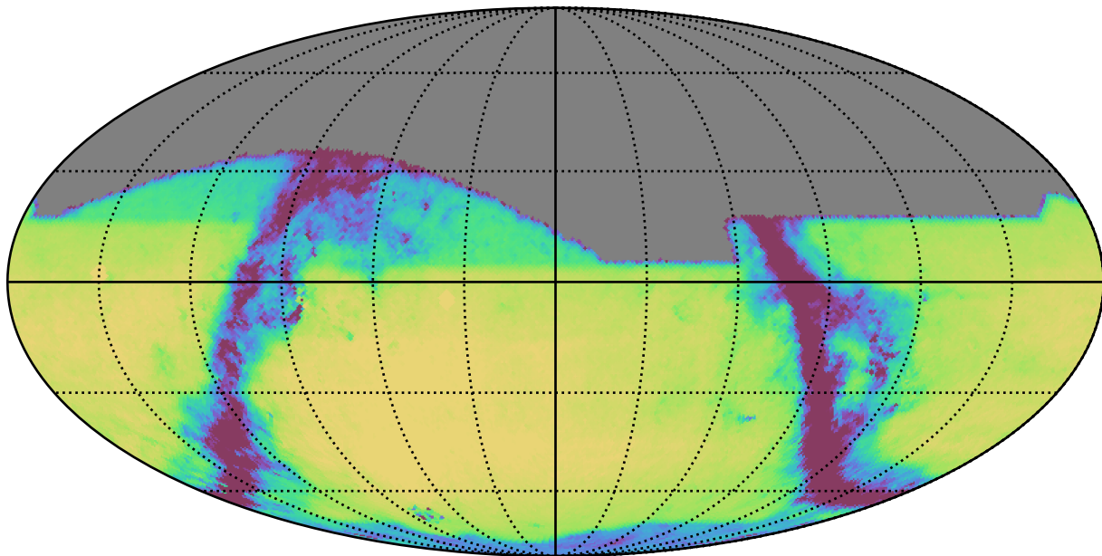
too_100_1v3.4_10yrs All sky r band: Exgal_CoaddM5
