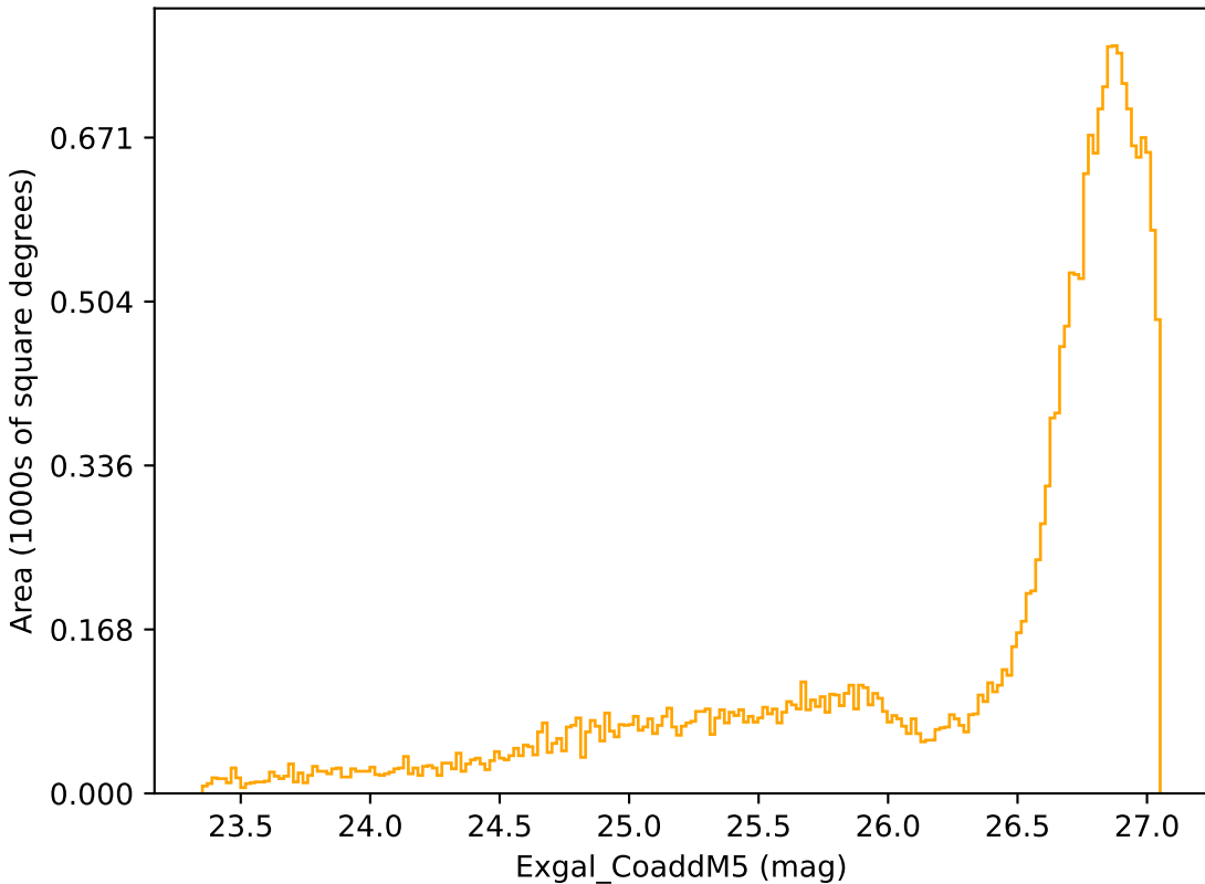
too_100_1v3.4_10yrs All sky r band: Exgal_CoaddM5
