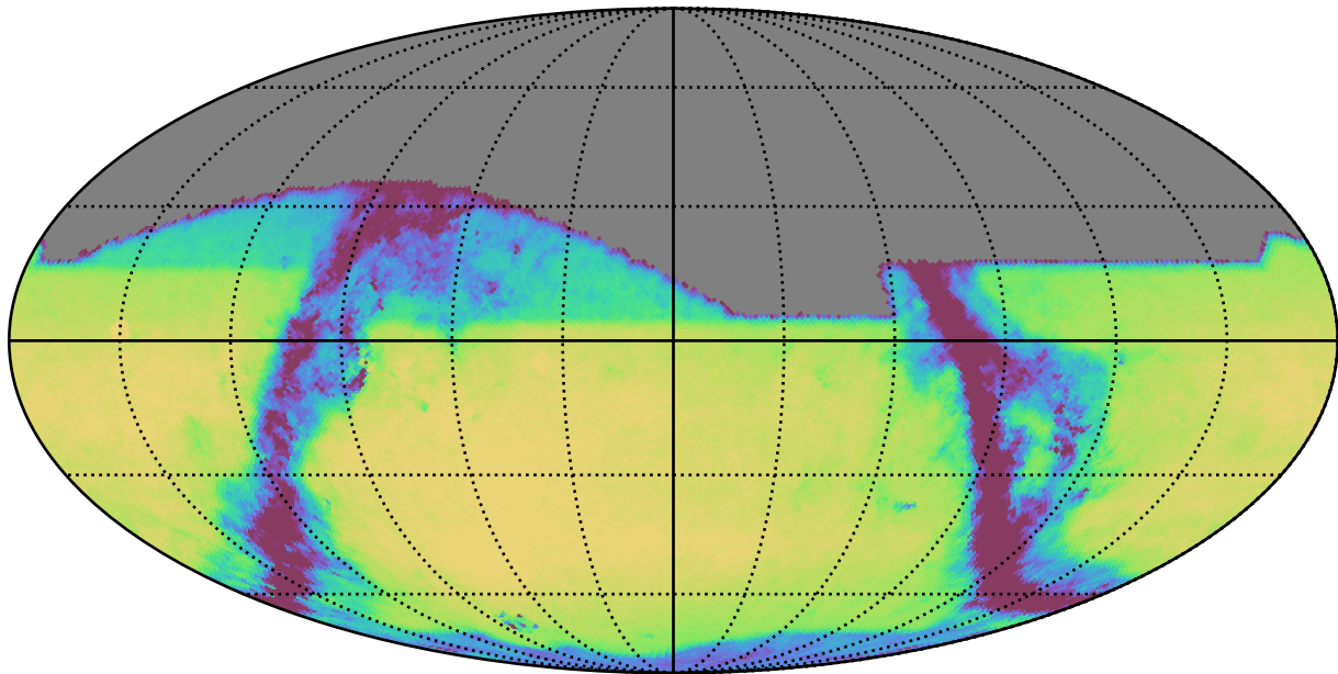
too_100_1v3.4_10yrs All sky i band: Exgal_CoaddM5
