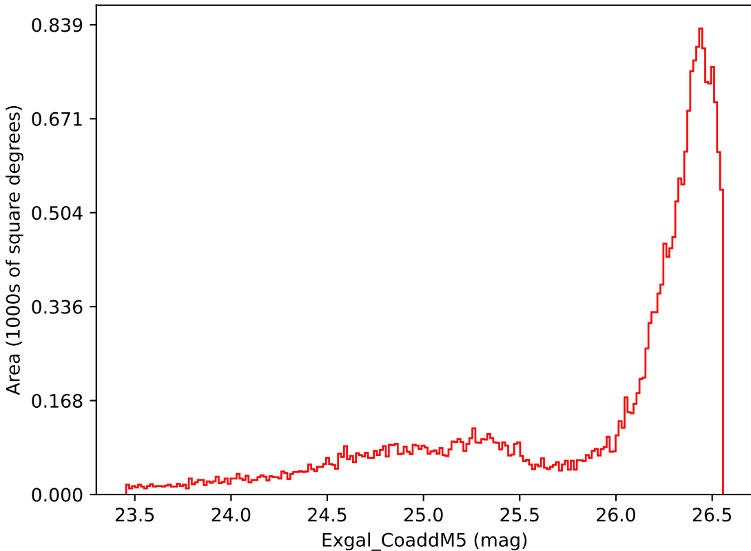
too_100_1v3.4_10yrs All sky i band: Exgal_CoaddM5
