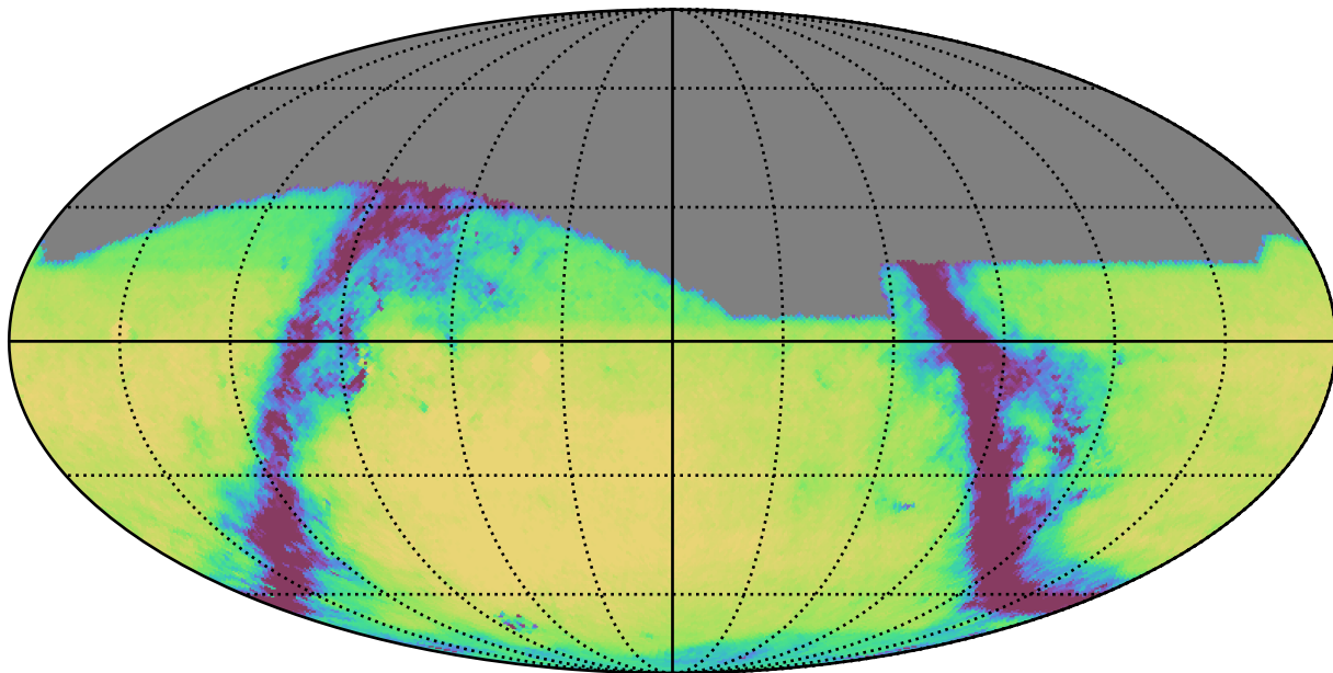
too_100_1v3.4_10yrs All sky g band: Exgal_CoaddM5
