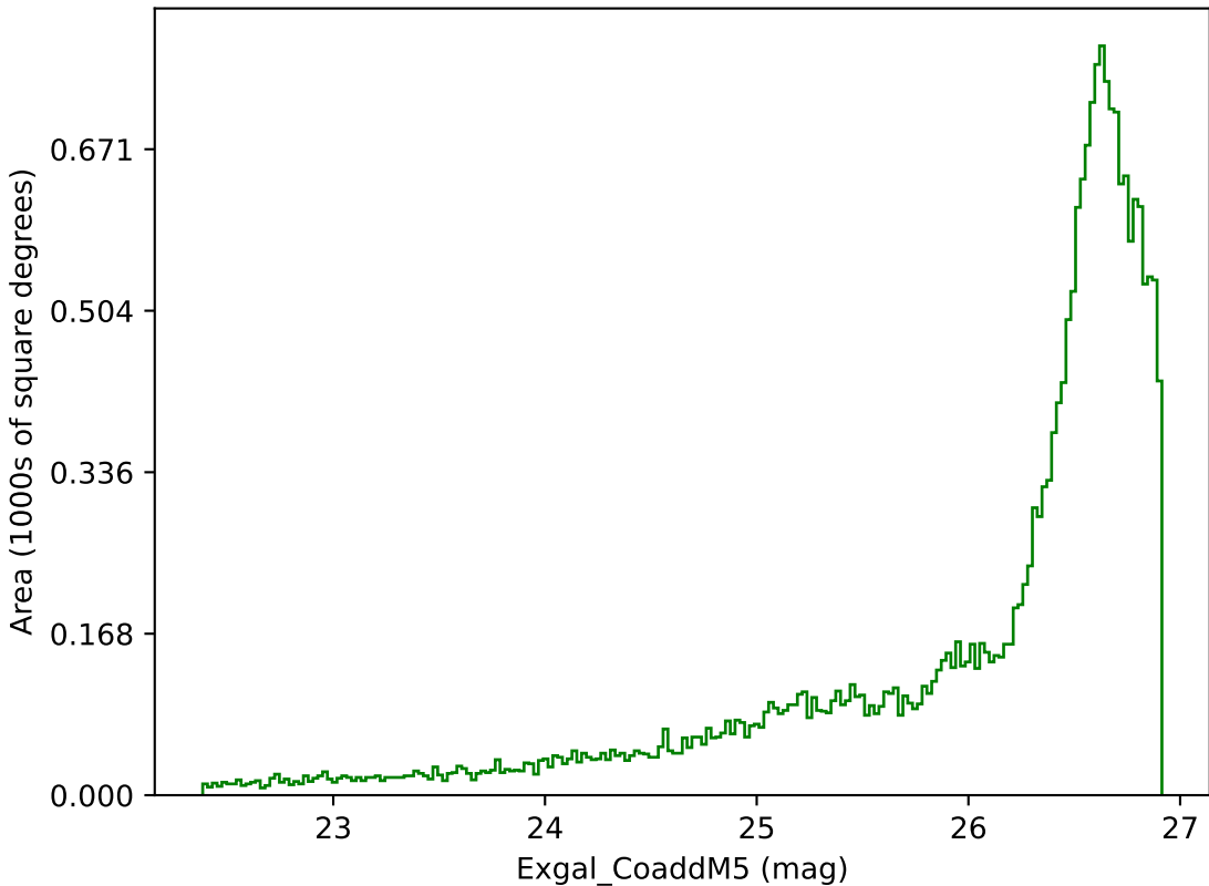
too_100_1v3.4_10yrs All sky g band: Exgal_CoaddM5
