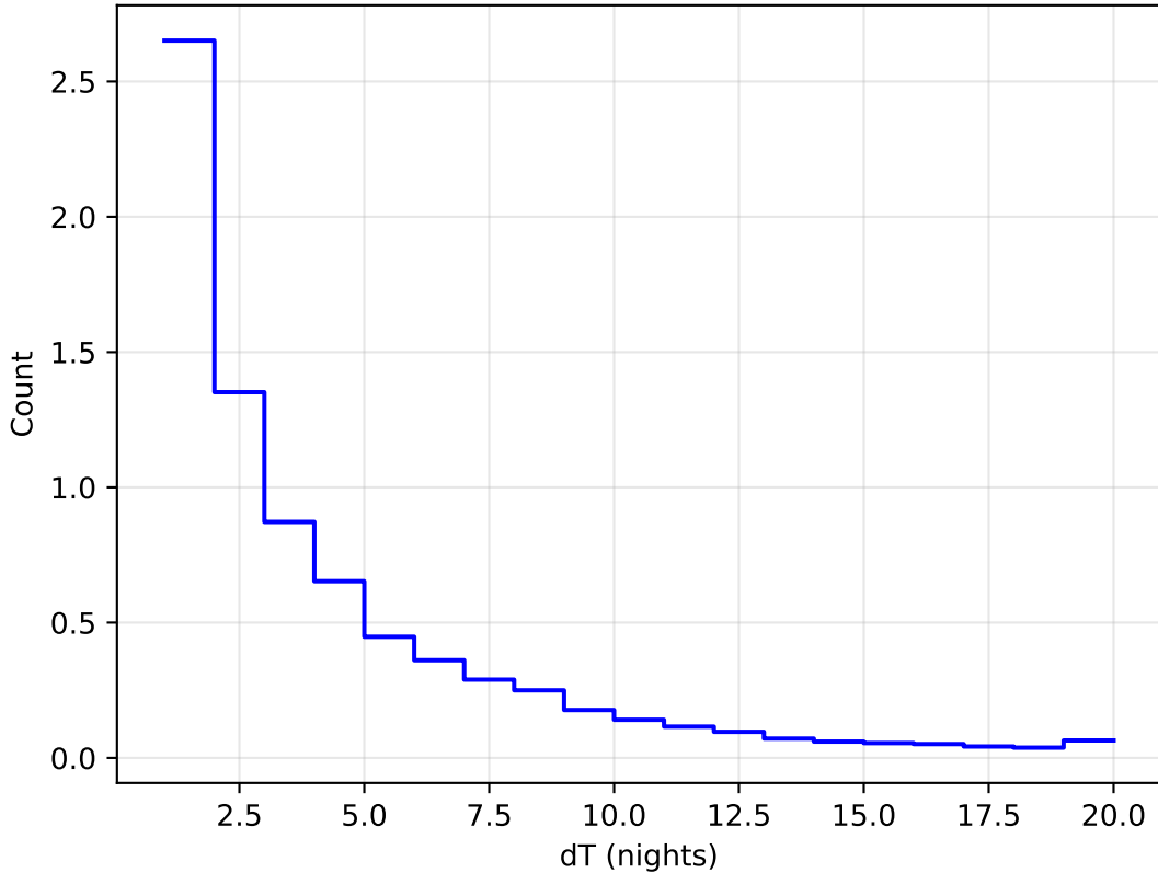
too_100_1v3.4_10yrs WFD all bands: DeltaNight Histogram 1e6
