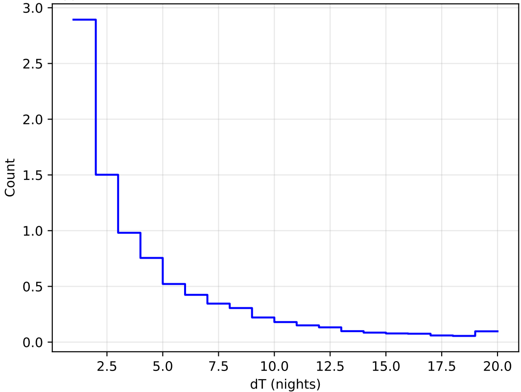
too_100_1v3.4_10yrs All sky all bands: DeltaNight Histogram 1e6
