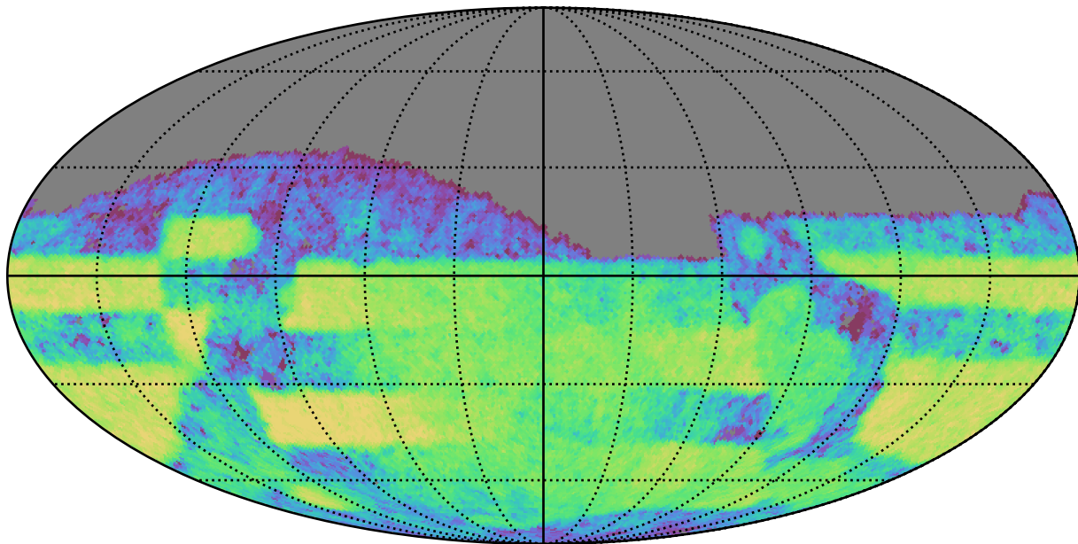
too_100_1v3.4_10yrs Yr 3-4 z band: CoaddM5
