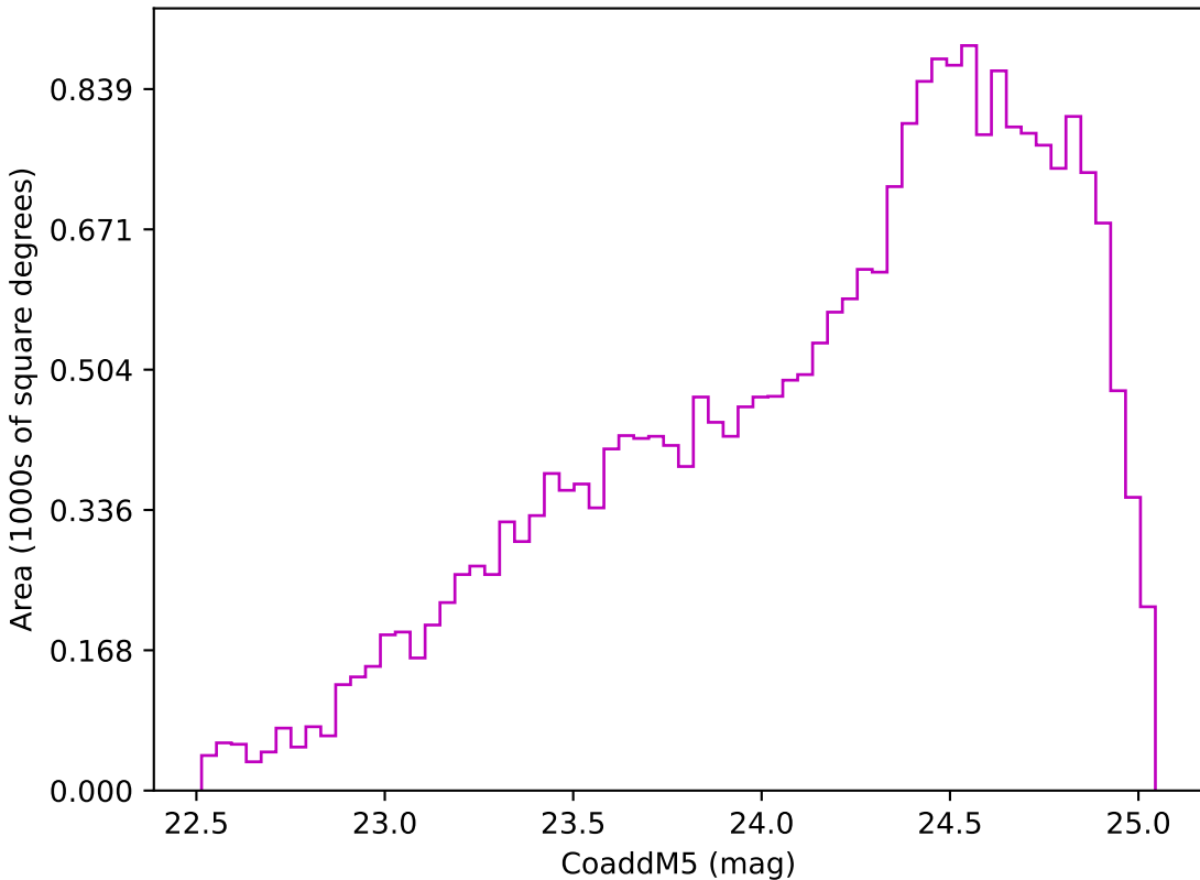
too_100_1v3.4_10yrs Yr 3-4 z band: CoaddM5
