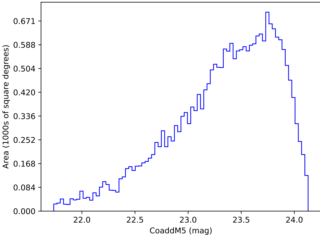
too_100_1v3.4_10yrs Yr 3-4 y band: CoaddM5
