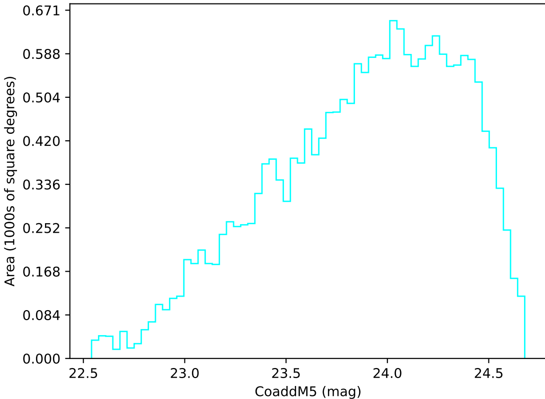
too_100_1v3.4_10yrs Yr 3-4 u band: CoaddM5
