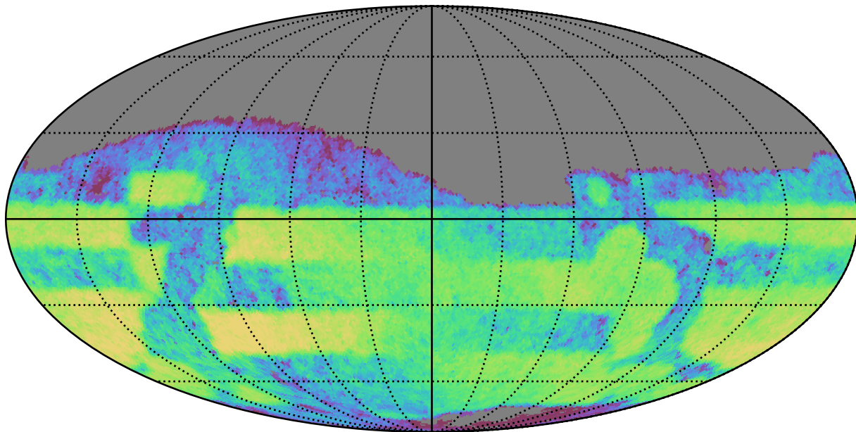
too_100_1v3.4_10yrs Yr 3-4 r band: CoaddM5
