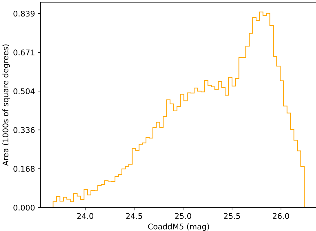
too_100_1v3.4_10yrs Yr 3-4 r band: CoaddM5
