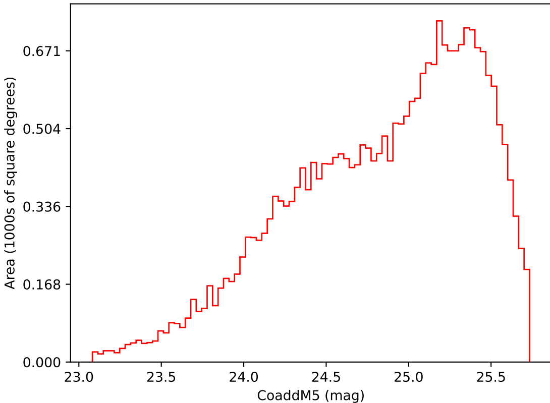
too_100_1v3.4_10yrs Yr 3-4 i band: CoaddM5
