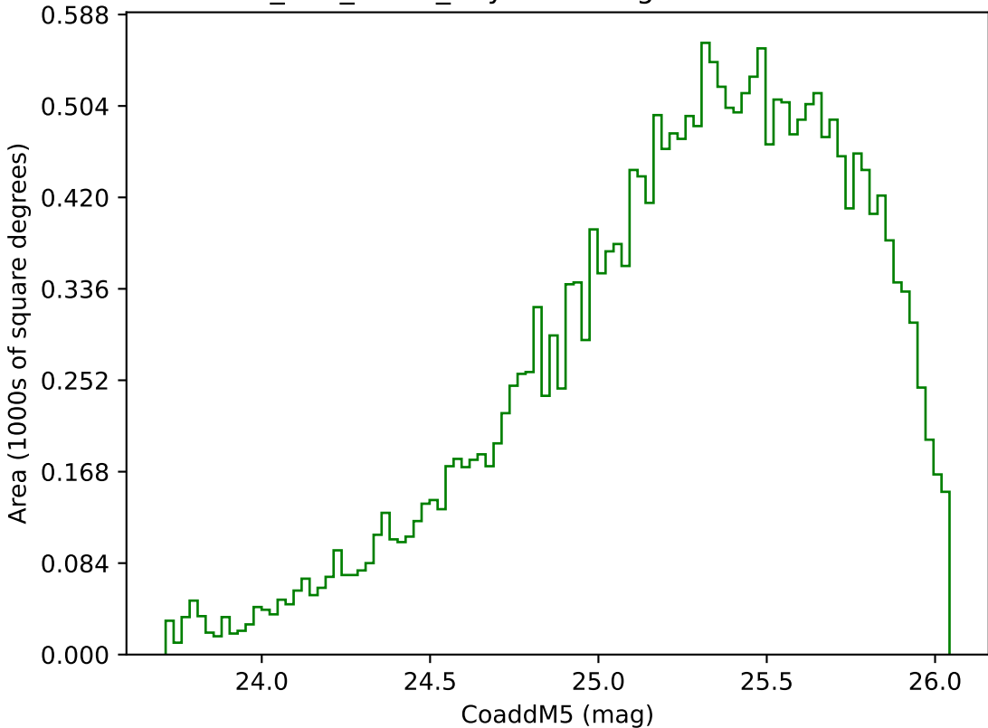
too_100_1v3.4_10yrs Yr 3-4 g band: CoaddM5
