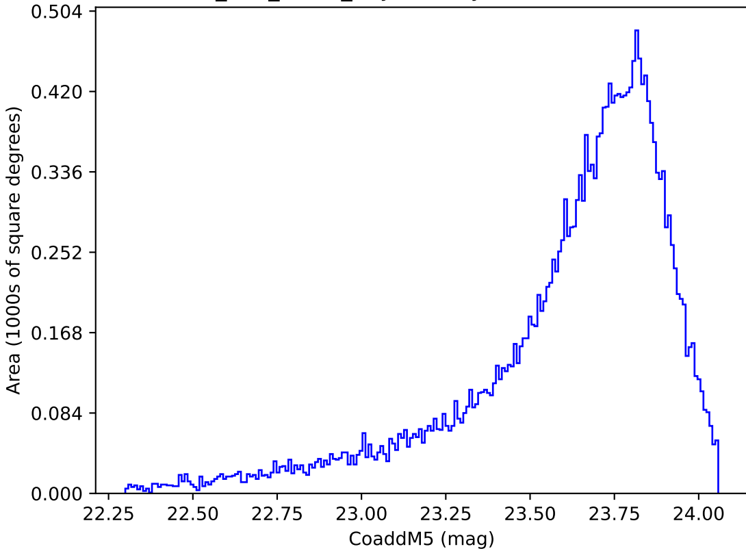
too_100_1v3.4_10yrs Yr 1 y band: CoaddM5
