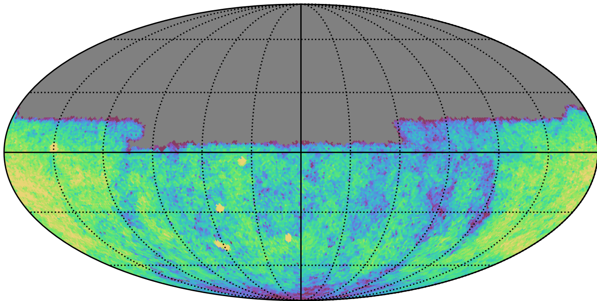
too_100_1v3.4_10yrs Yr 1 u band: CoaddM5
