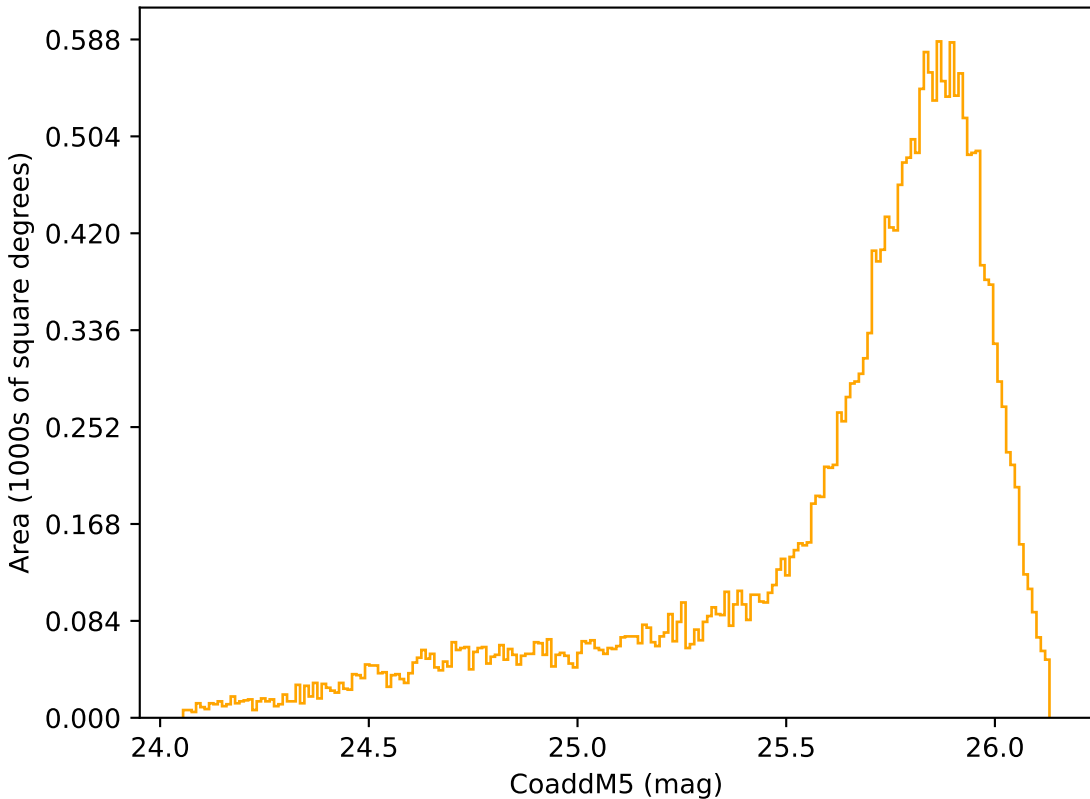
too_100_1v3.4_10yrs Yr 1 r band: CoaddM5
