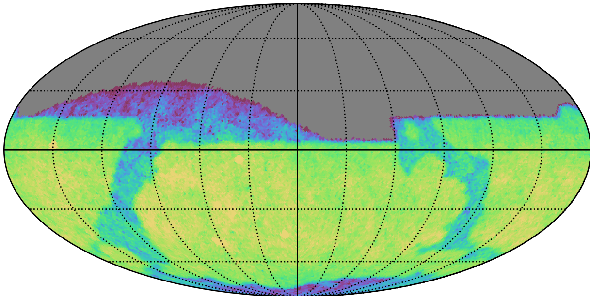
too_100_1v3.4_10yrs Yr 1 i band: CoaddM5
