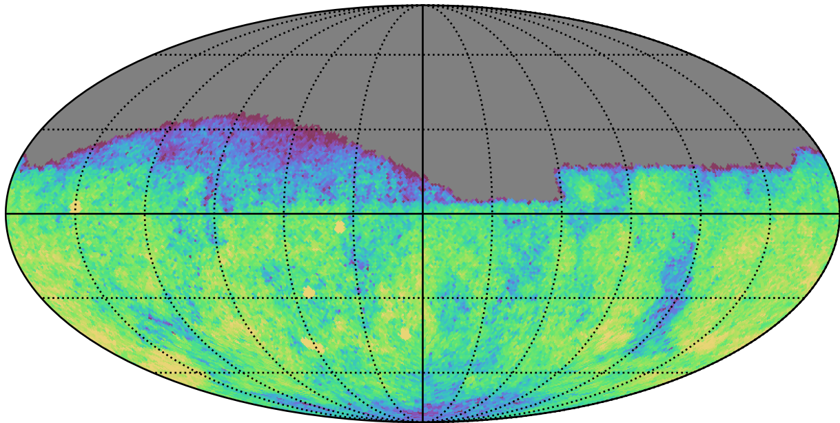
too_100_1v3.4_10yrs Yr 1 g band: CoaddM5
