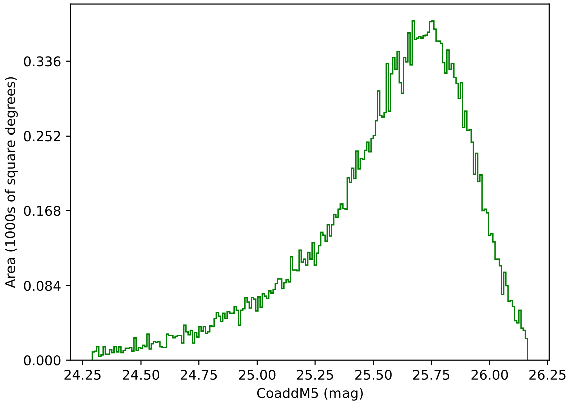
too_100_1v3.4_10yrs Yr 1 g band: CoaddM5
