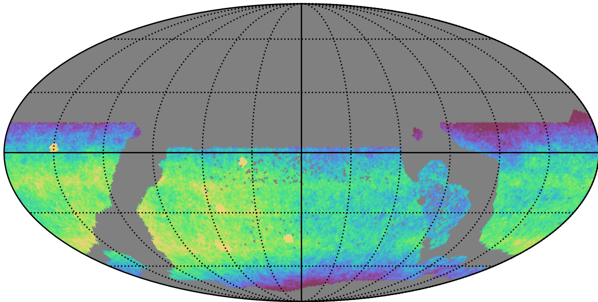
too_100_1v3.4_10yrs WFD z band: CoaddM5
