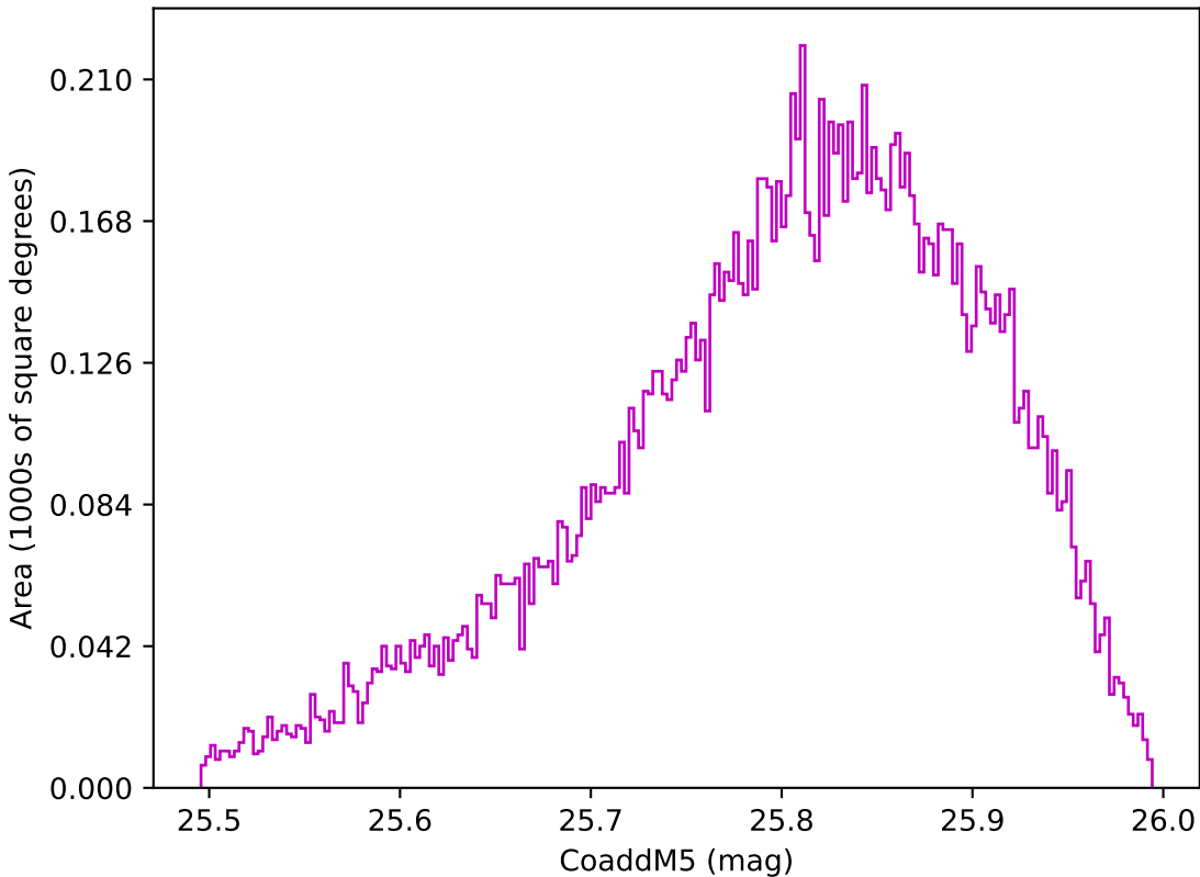
too_100_1v3.4_10yrs WFD z band: CoaddM5
