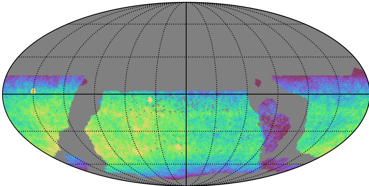
too_100_1v3.4_10yrs WFD y band: CoaddM5
