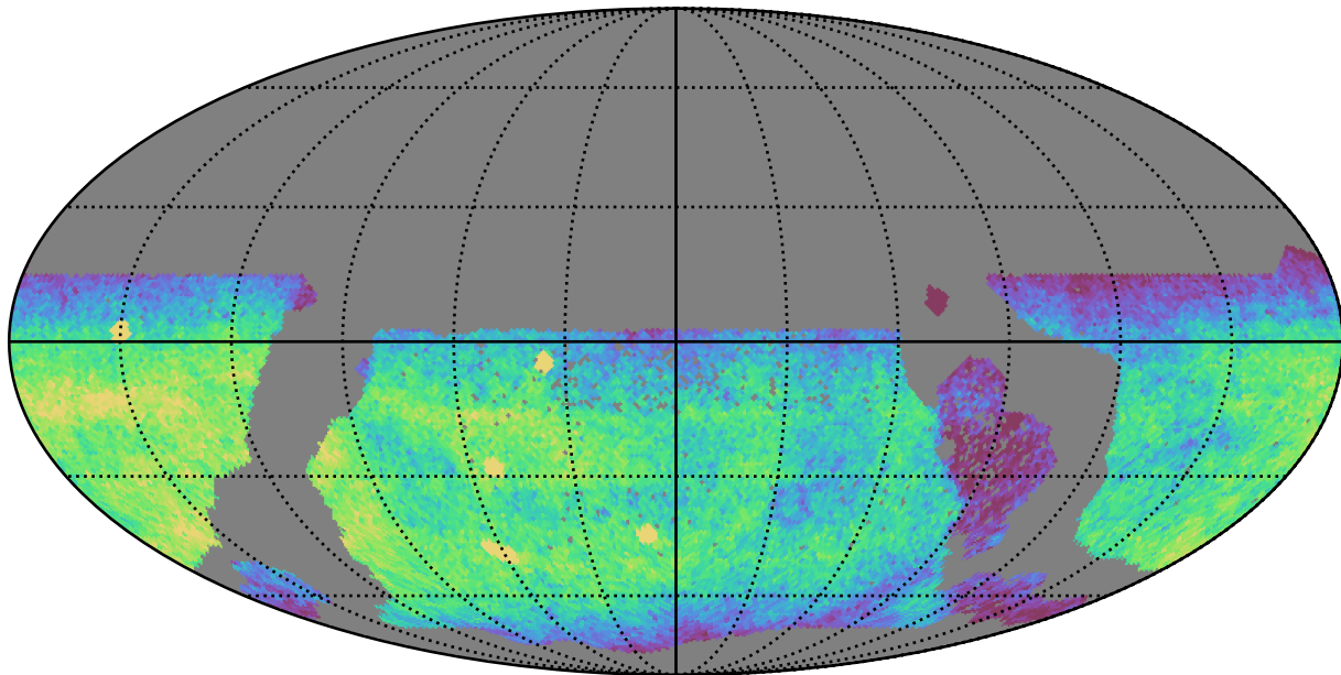
too_100_1v3.4_10yrs WFD u band: CoaddM5
