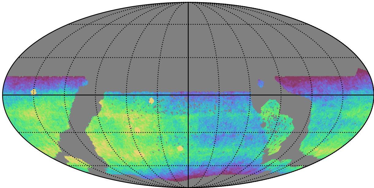
too_100_1v3.4_10yrs WFD r band: CoaddM5
