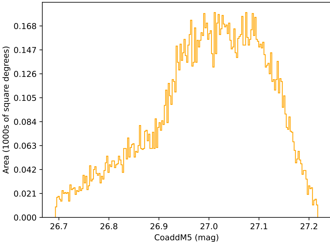
too_100_1v3.4_10yrs WFD r band: CoaddM5
