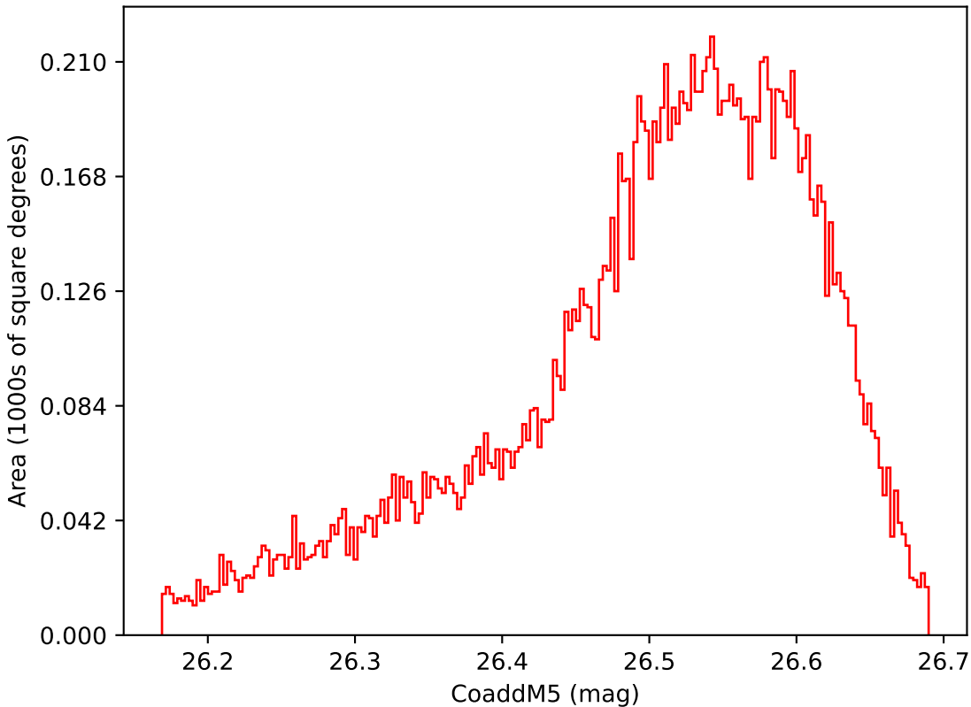
too_100_1v3.4_10yrs WFD i band: CoaddM5
