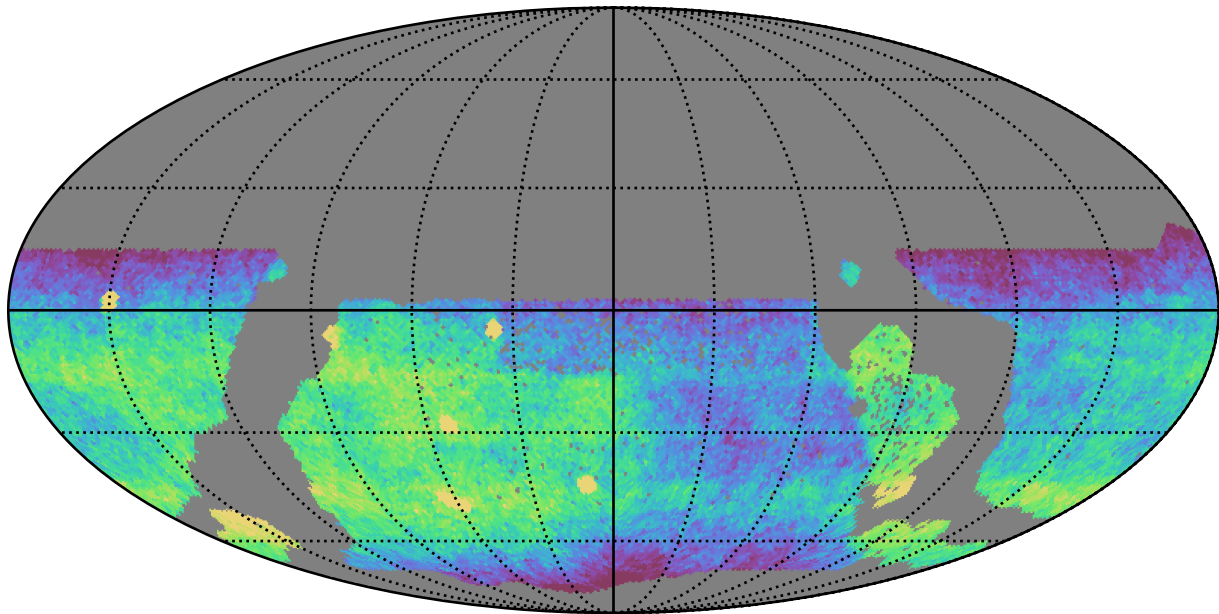
too_100_1v3.4_10yrs WFD g band: CoaddM5
