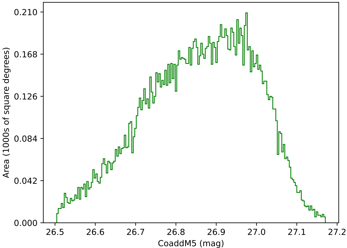
too_100_1v3.4_10yrs WFD g band: CoaddM5
