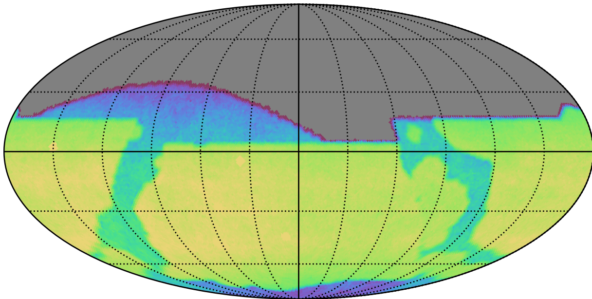
too_100_1v3.4_10yrs All sky z band: CoaddM5
