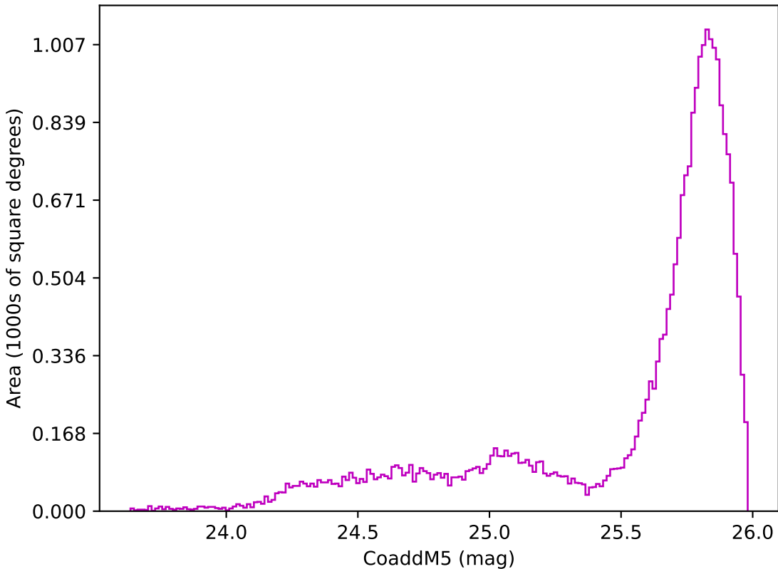
too_100_1v3.4_10yrs All sky z band: CoaddM5
