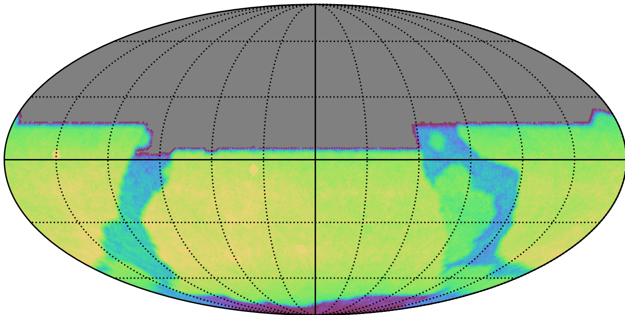
too_100_1v3.4_10yrs All sky y band: CoaddM5
