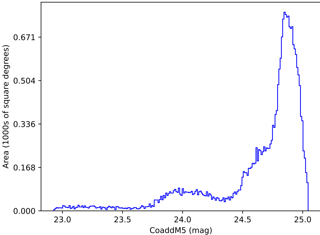
too_100_1v3.4_10yrs All sky y band: CoaddM5
