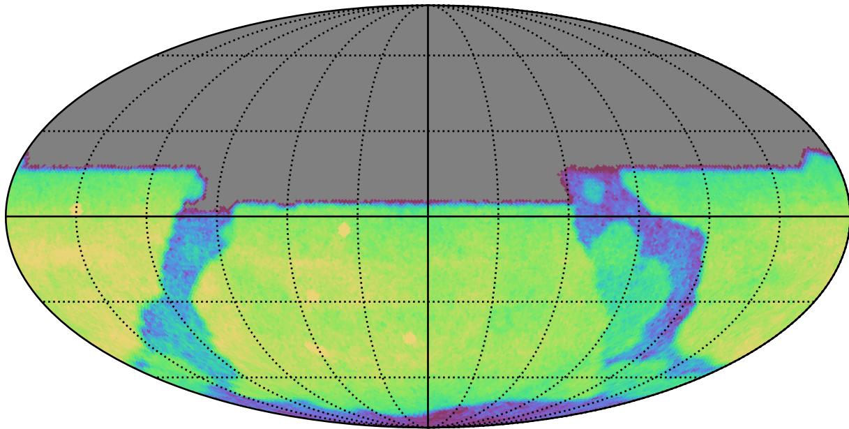
too_100_1v3.4_10yrs All sky u band: CoaddM5
