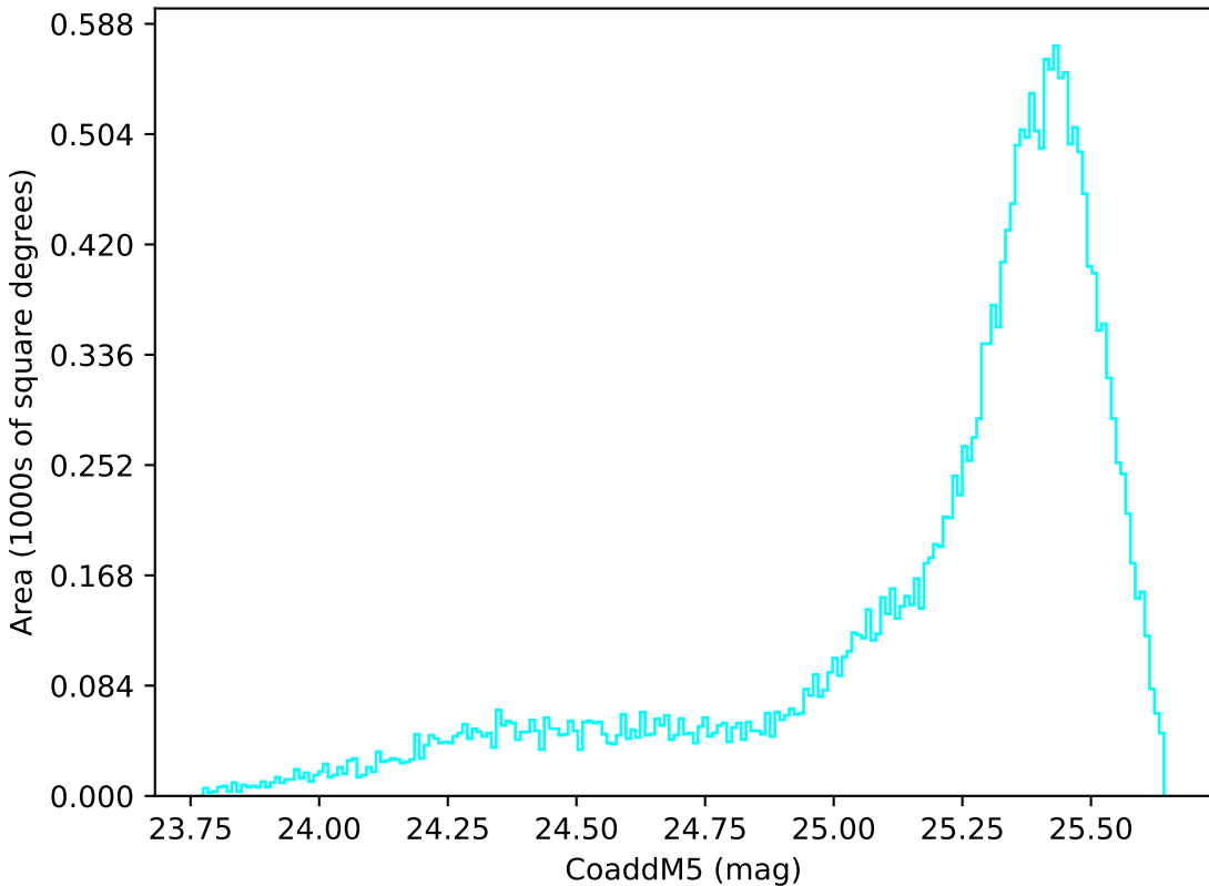
too_100_1v3.4_10yrs All sky u band: CoaddM5
