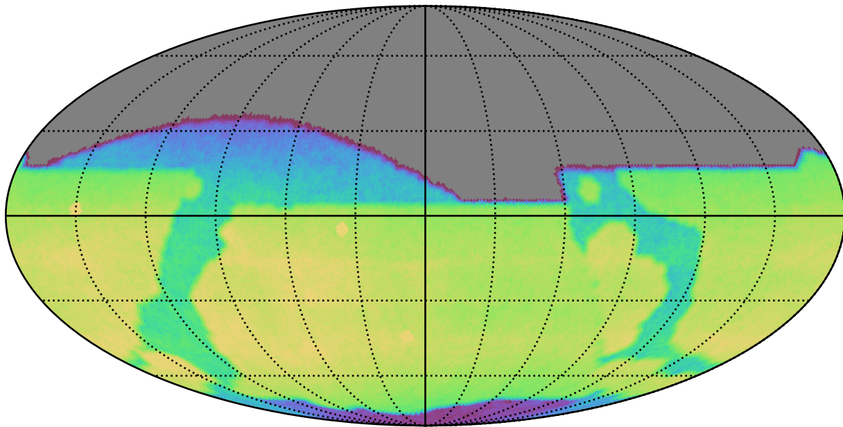
too_100_1v3.4_10yrs All sky r band: CoaddM5
