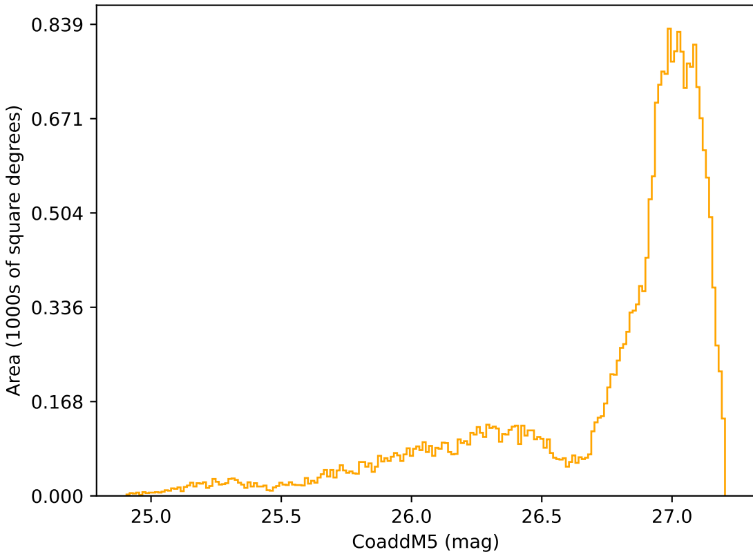
too_100_1v3.4_10yrs All sky r band: CoaddM5
