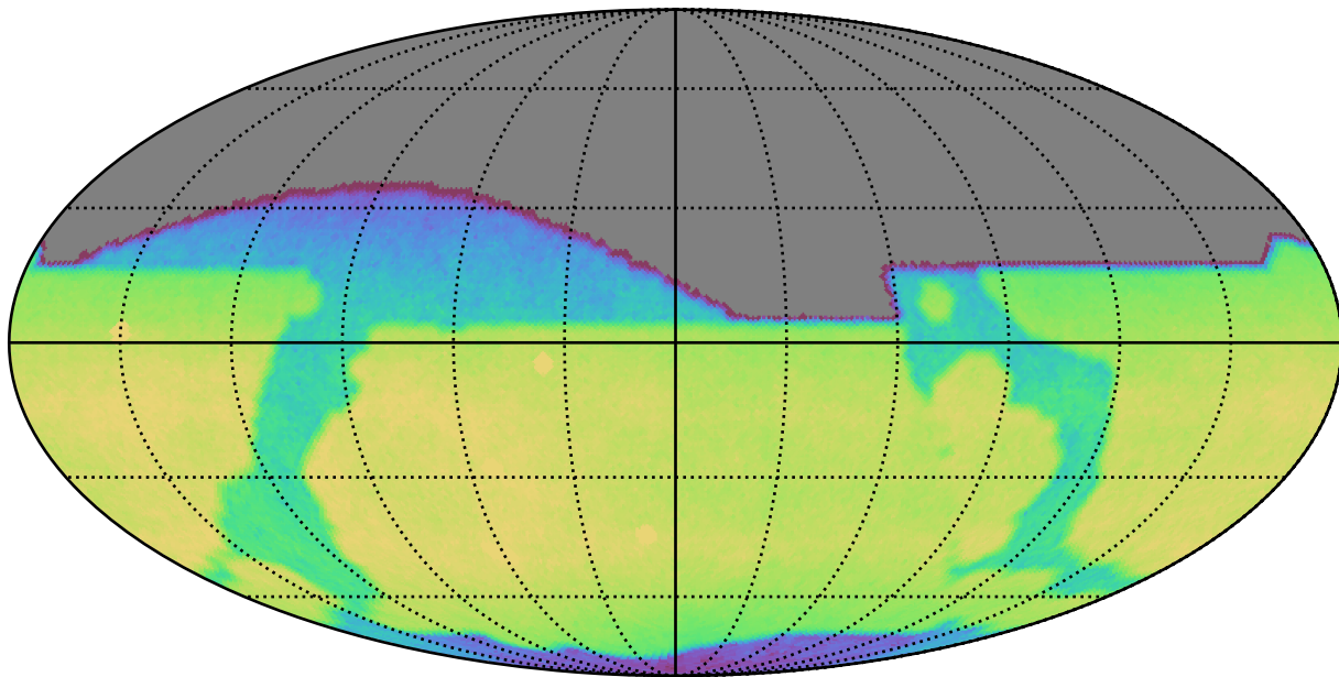
too_100_1v3.4_10yrs All sky i band: CoaddM5
