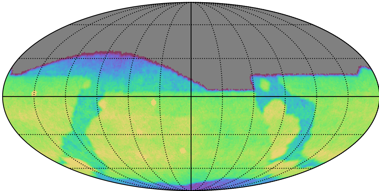
too_100_1v3.4_10yrs All sky g band: CoaddM5
