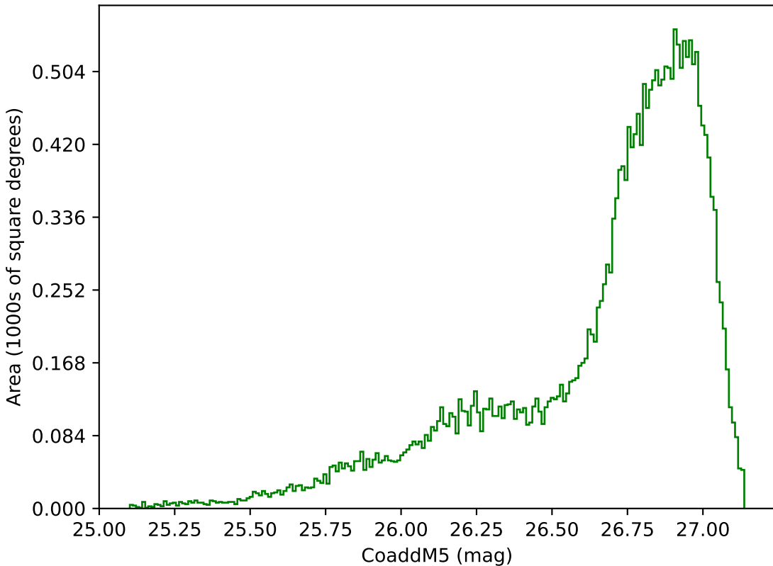
too_100_1v3.4_10yrs All sky g band: CoaddM5
