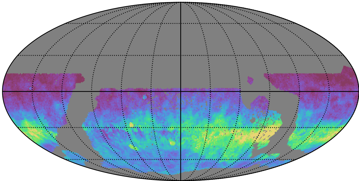
too_100_1v3.4_10yrs WFD z band: AngleRms rotSkyPos
