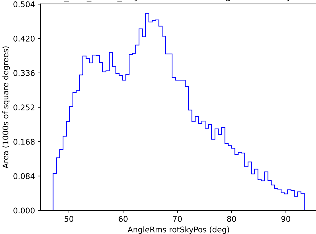
too_100_1v3.4_10yrs WFD z band: AngleRms rotSkyPos
