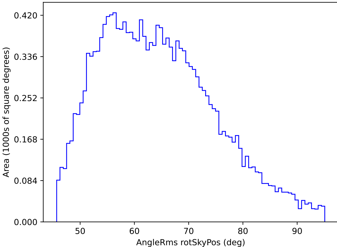
too_100_1v3.4_10yrs WFD u band: AngleRms rotSkyPos
