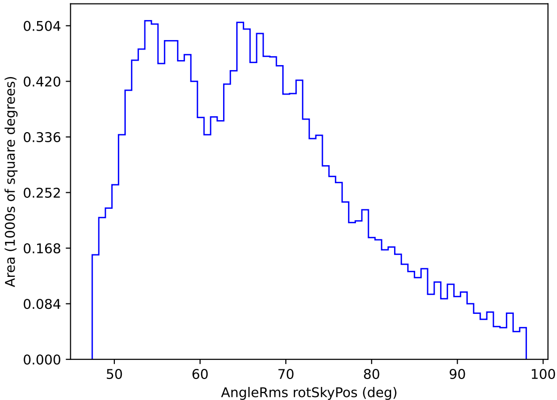
too_100_1v3.4_10yrs WFD r band: AngleRms rotSkyPos
