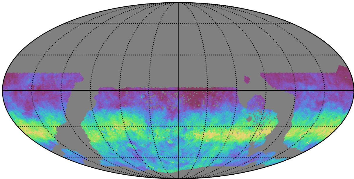
too_100_1v3.4_10yrs WFD g band: AngleRms rotSkyPos
