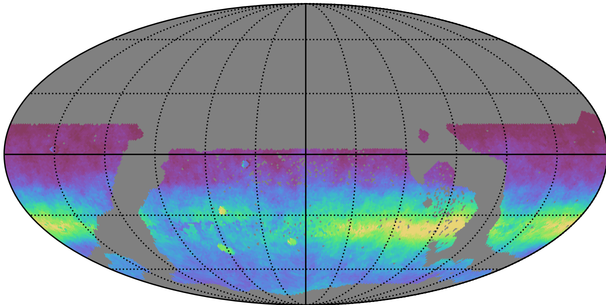
too_100_1v3.4_10yrs WFD all bands: AngleRms rotSkyPos
