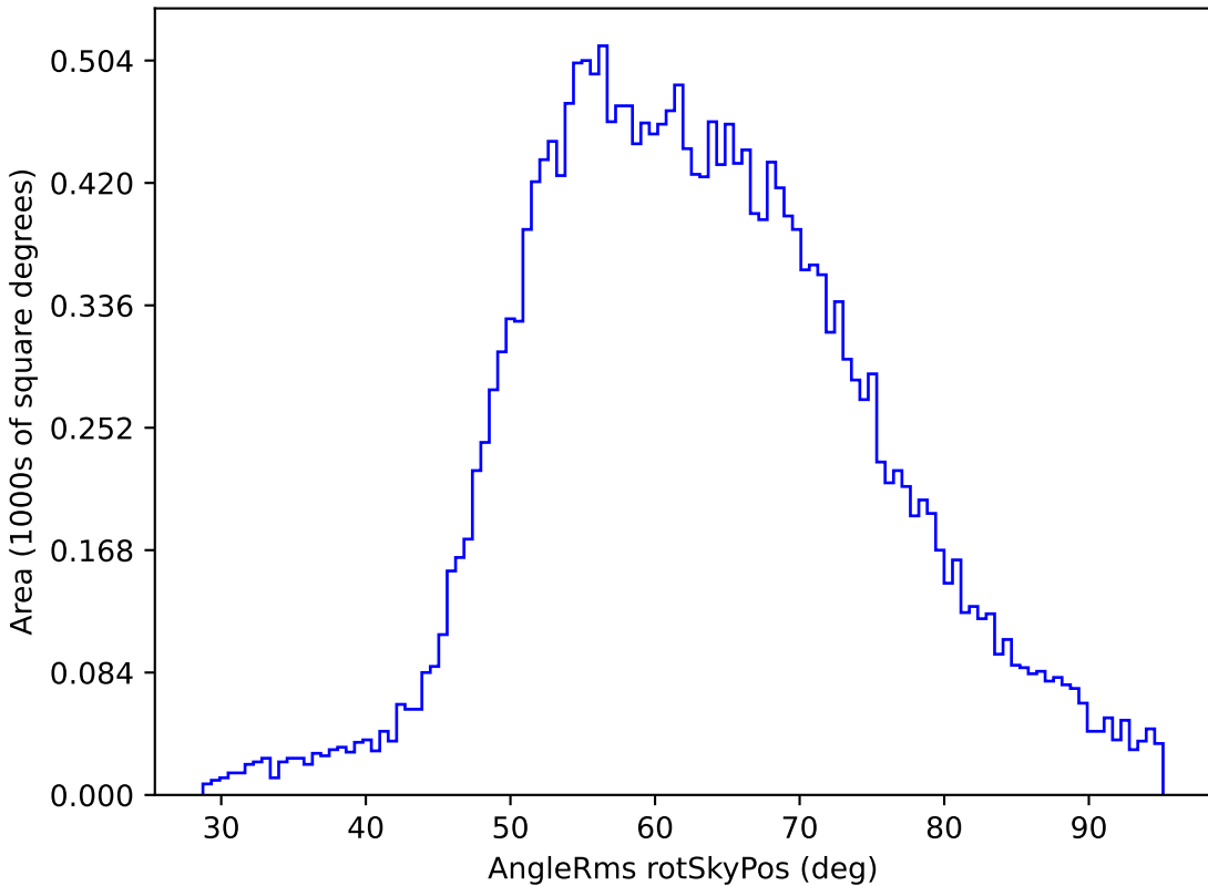
too_100_1v3.4_10yrs All sky u band: AngleRms rotSkyPos
