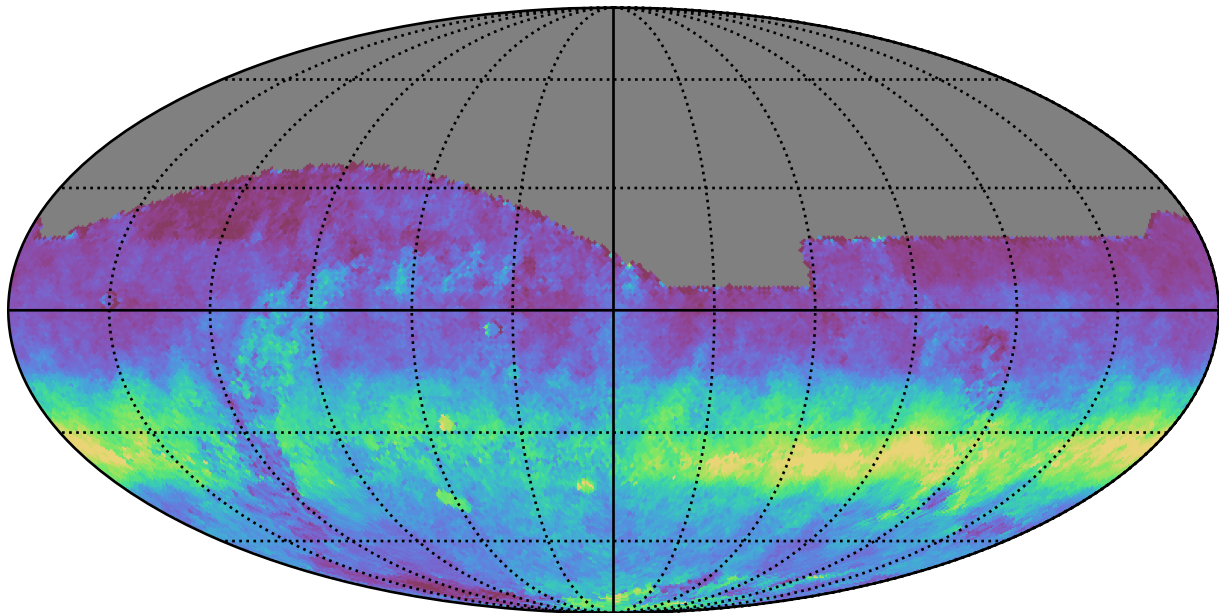
too_100_1v3.4_10yrs All sky r band: AngleRms rotSkyPos
